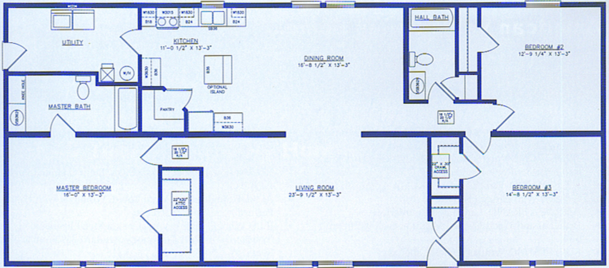
Huntington Floor Plan
