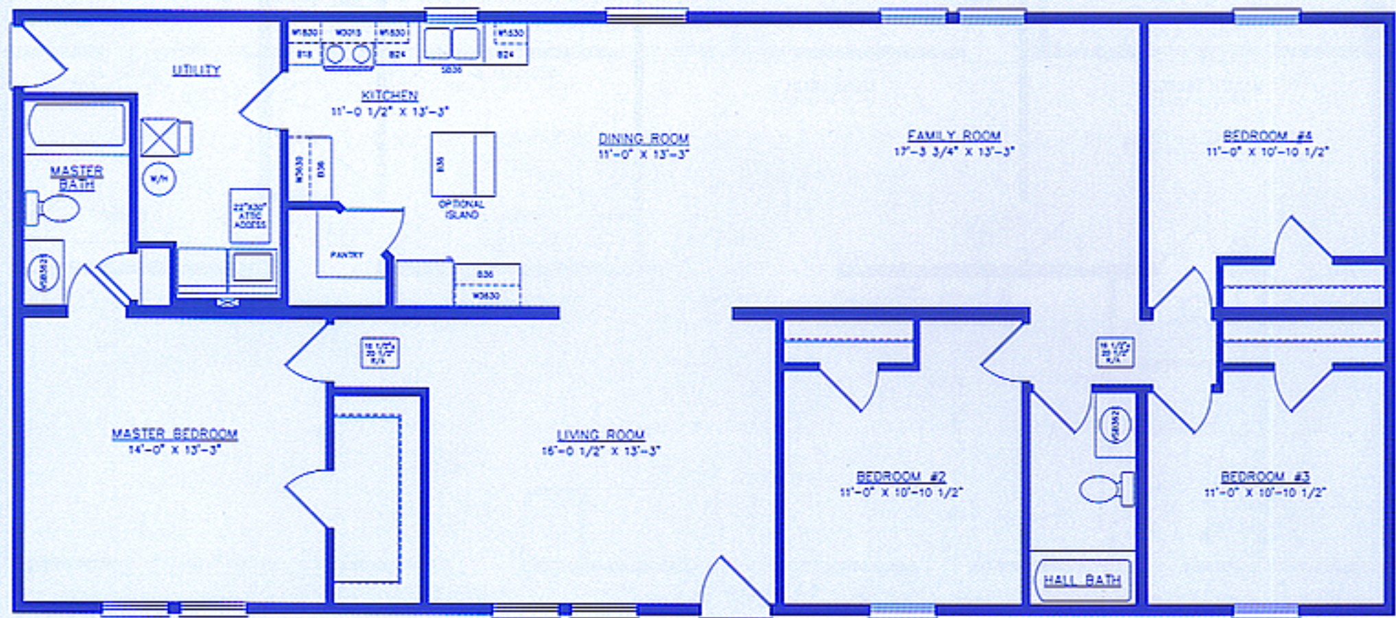
Anderson Floor Plan
